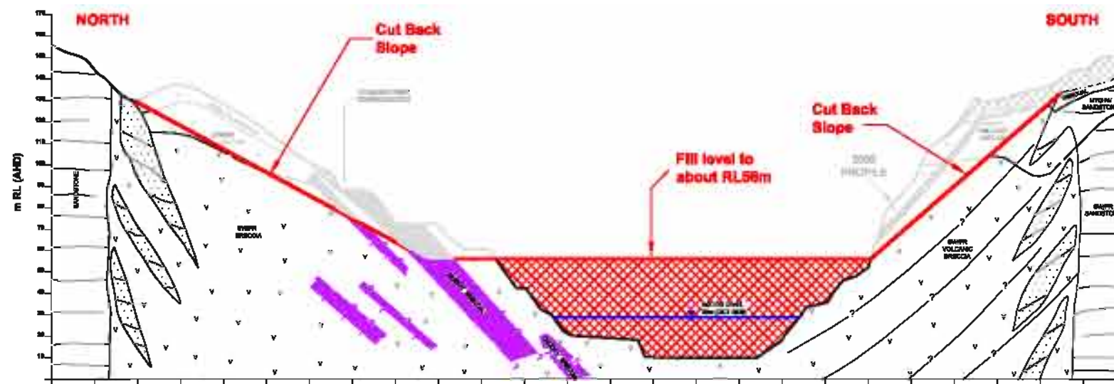
CONCEPTUAL SECTION NORTH TO SOUTH
