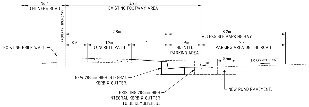
ACCESSIBLE BAY - TYPICAL SECTION NOT TO SCALE
