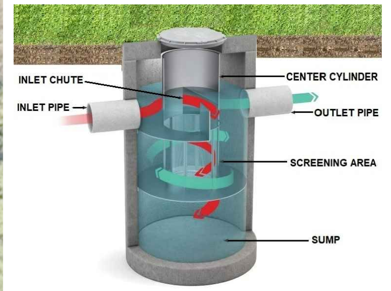
TYPICAL GROSS POLLUTANT TRAP
