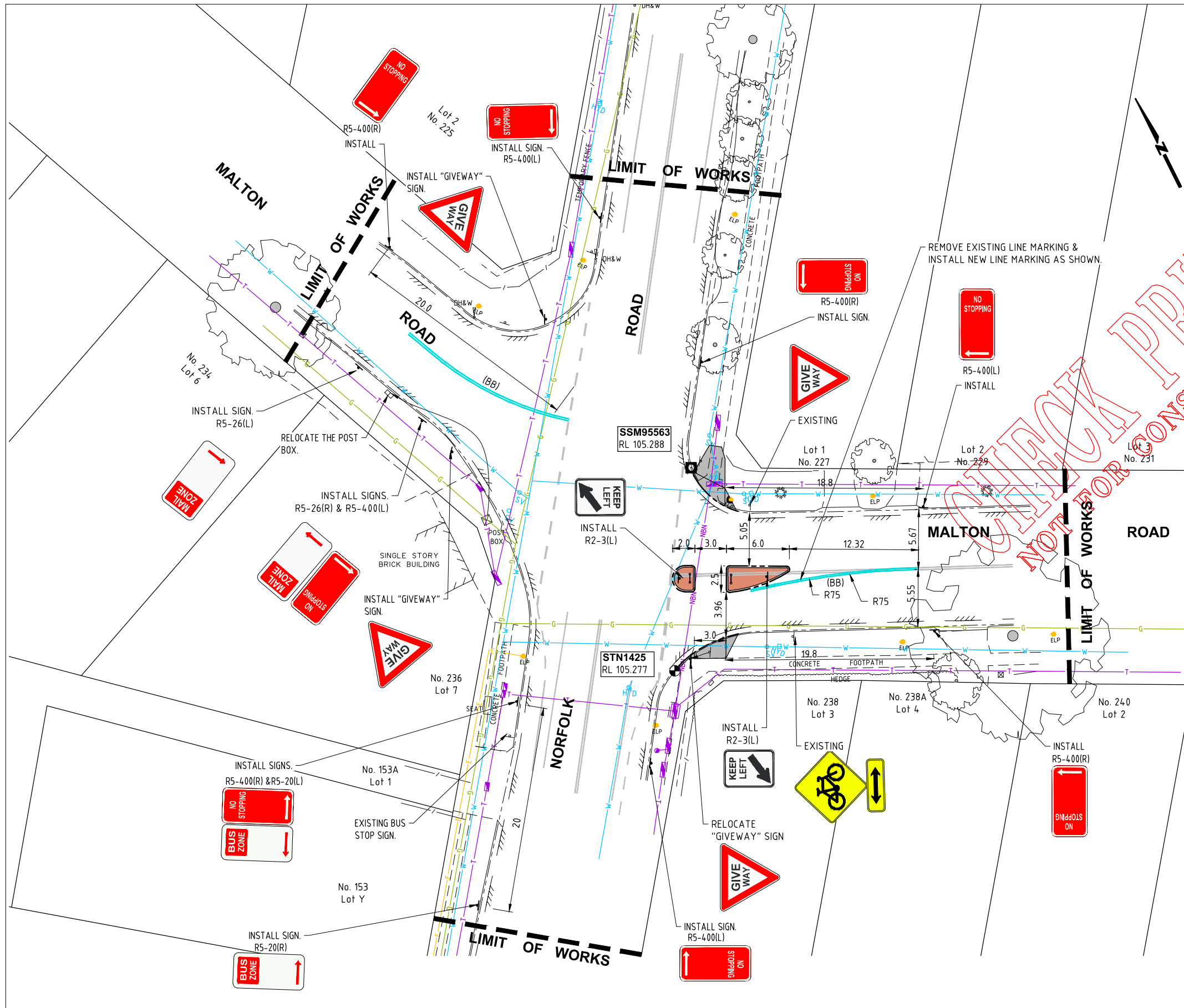
SIGNS & LINE MARKING PLAN SCALE 1:200
