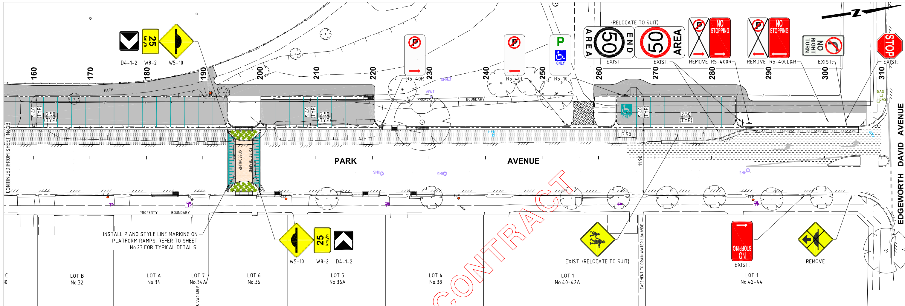
SIGNS & LINE MARKING PLAN
