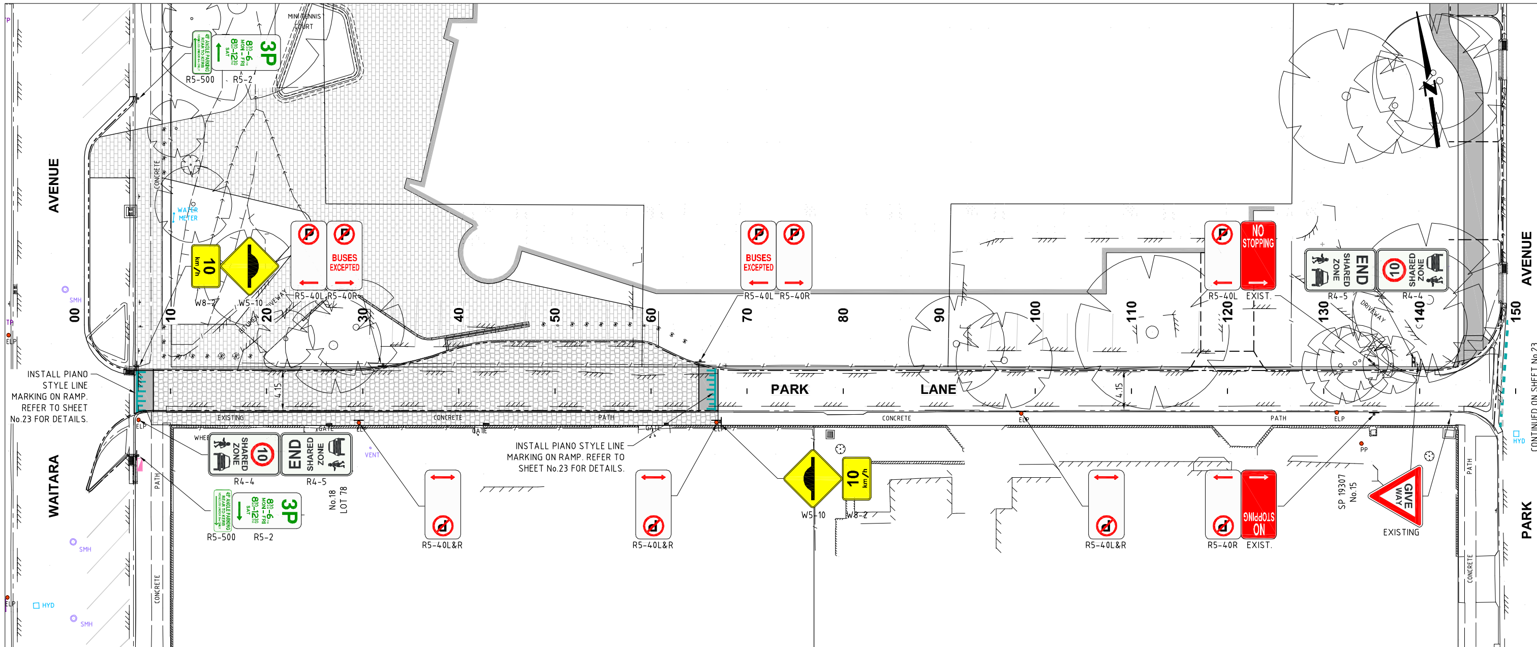
SIGNS & LINE MARKING PLAN
