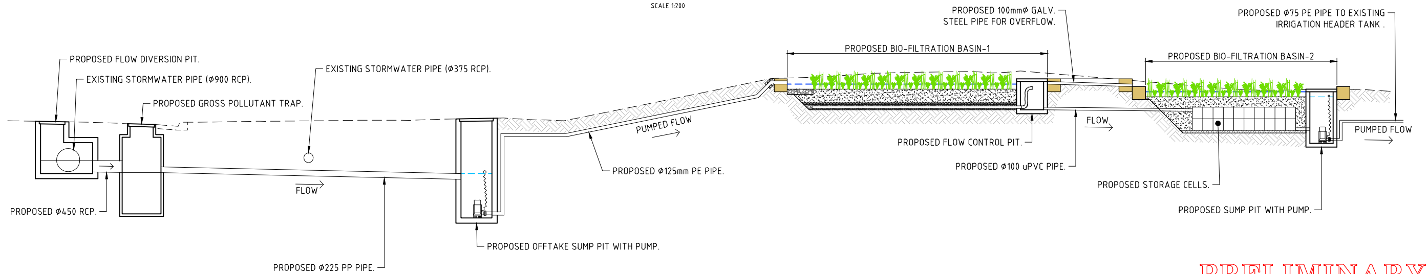
CONCEPT SECTION NOT TO SCALE
