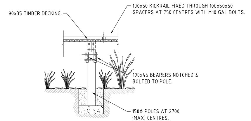
ISOMETRIC VIEW OF TIMBER BOARDWALK NOT TO SCALE
