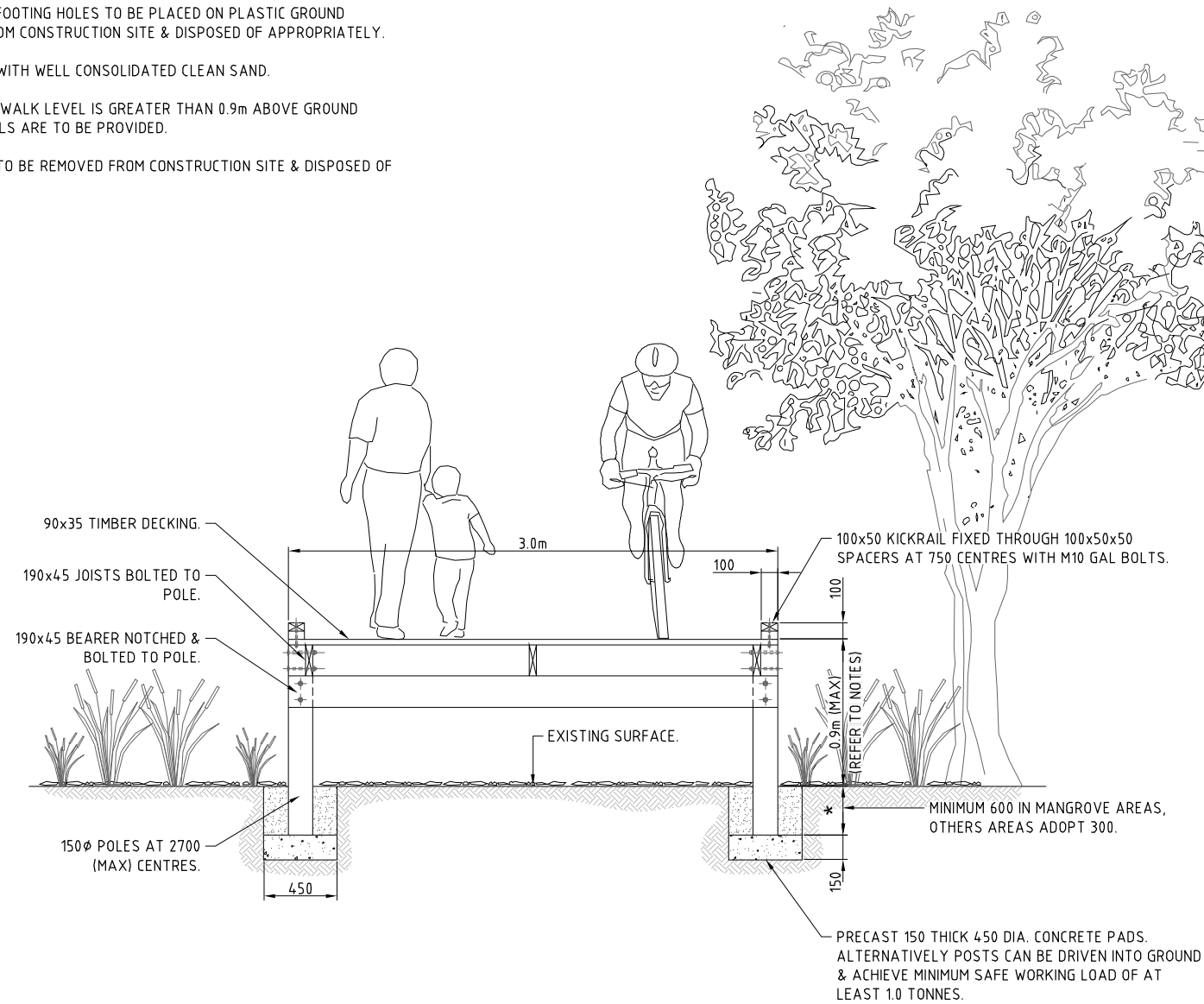
TYPICAL SECTION - TIMBER BOARDWALK NOT TO SCALE
